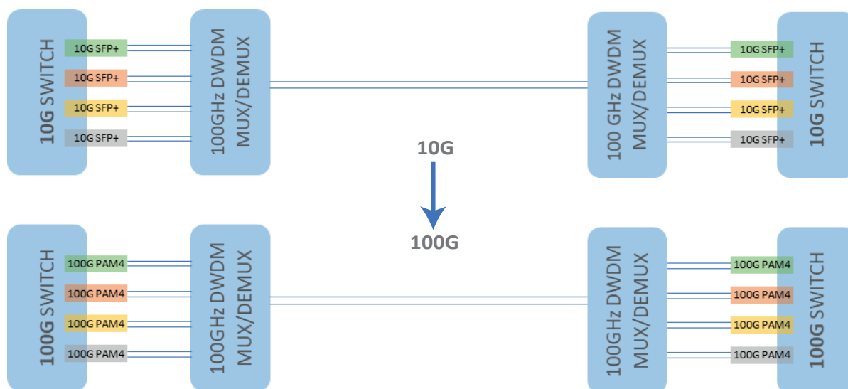
Figure 3 - 10G to 100G DWDM upgrade (100G PAM4 is on QSFP28 form factor and requires amplification)
